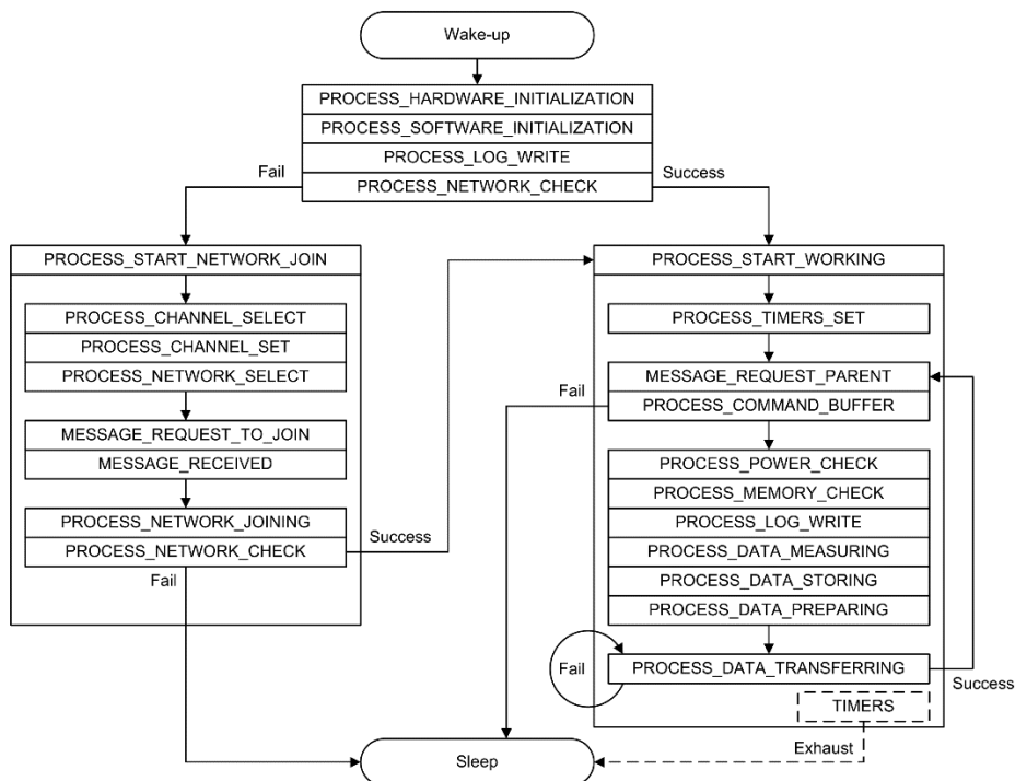
Fig. 4. Structure of applied software of measuring node
