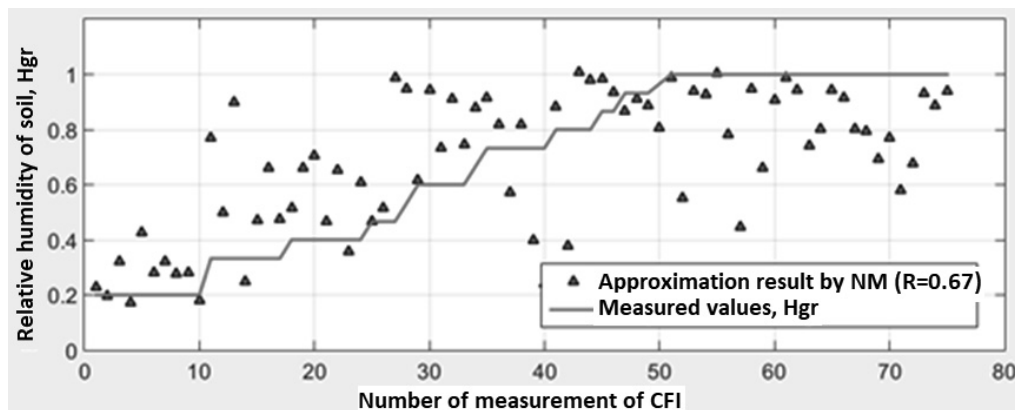
Fig. 7. Results of neural network approximation of the dependence of the chlorophyll fluorescence induction curve on soil moisture
