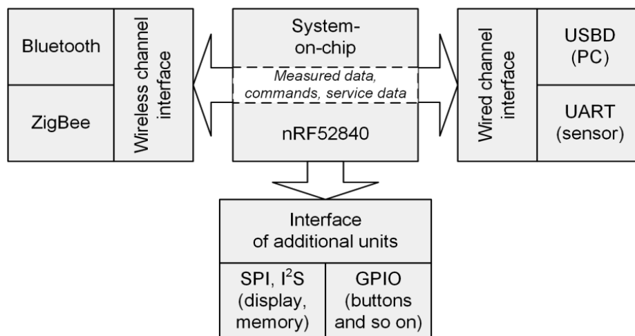
Fig. 2. The generalized structural diagram of the wireless communication module
