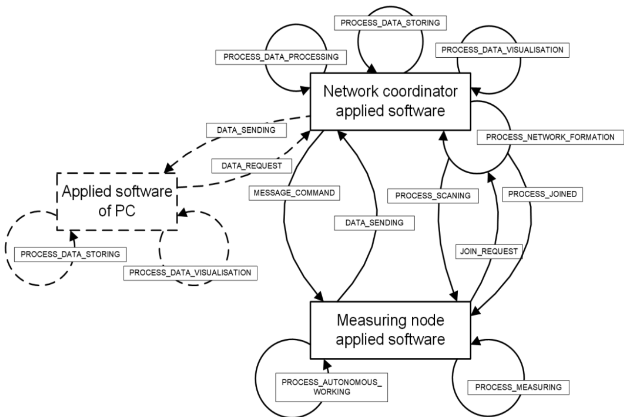
Fig. 5. The scheme of interaction of applied software of wireless nodes on the base of network coordinator
