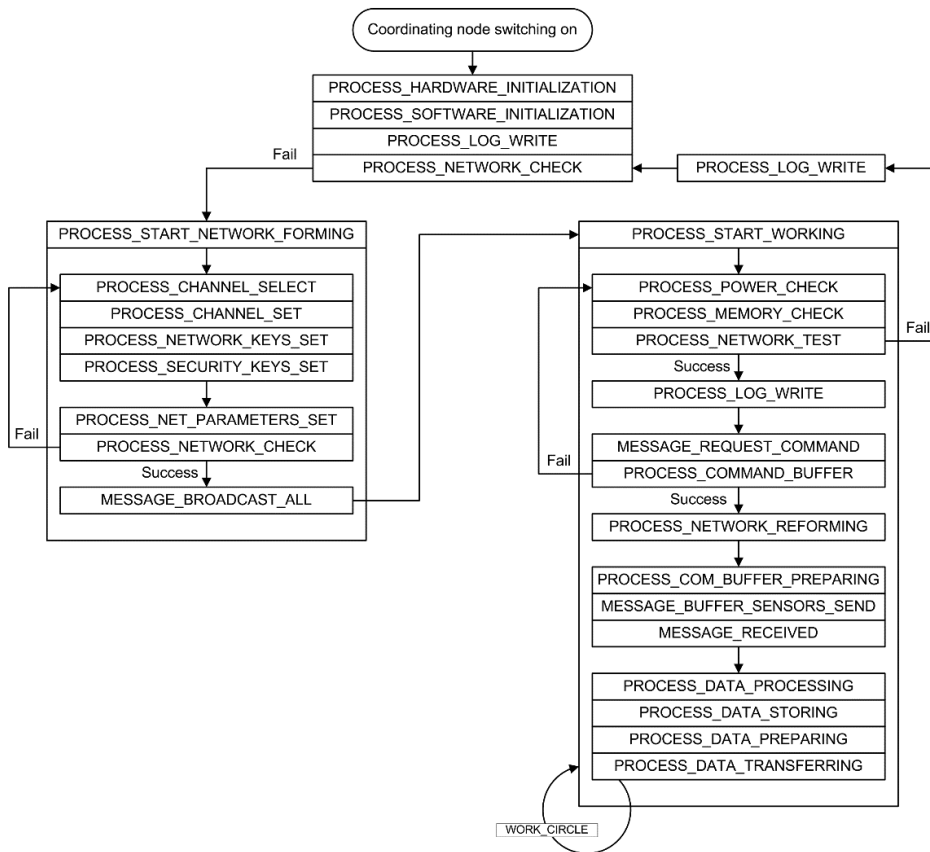
Fig. 3. Structure of applied software of network coordinator
