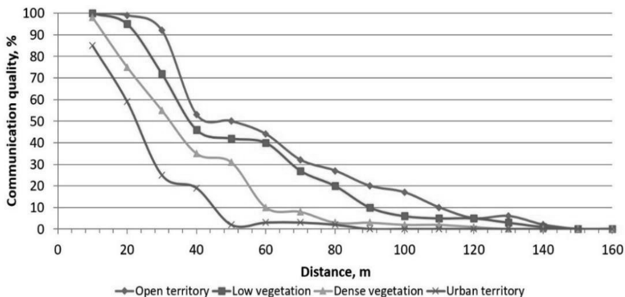
Fig. 8. The general dependence of coefficient of communication reliability (quality) on distance between network coordinator and wireless measuring node
